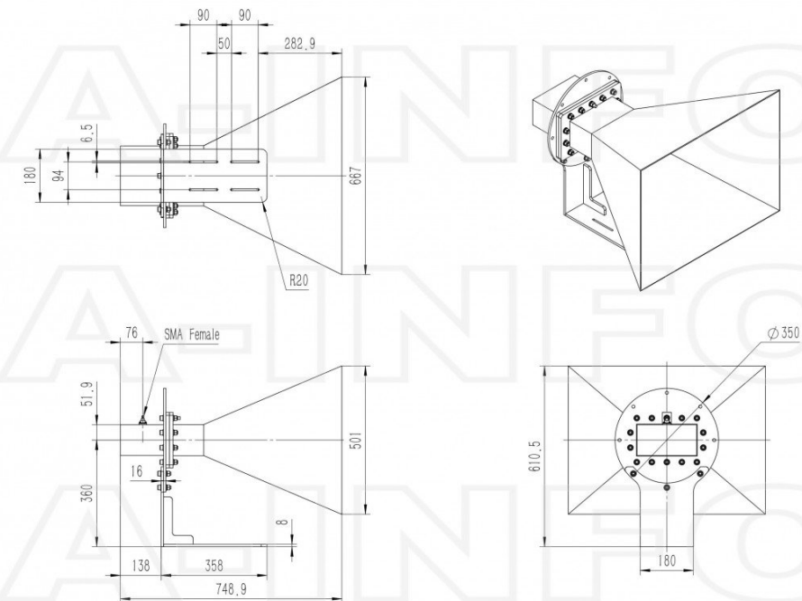
SMA Female Output with L Type Mounting Bracket (Option, P/N: LB-770-15-C-L)
