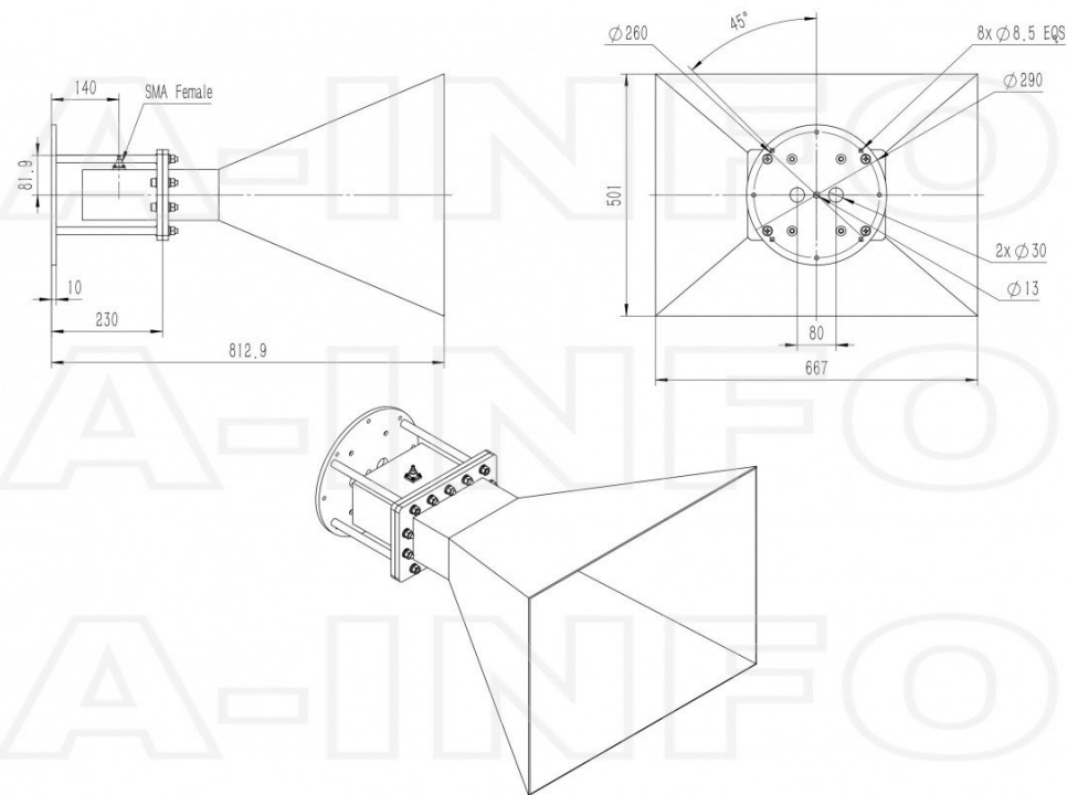
SMA Female Output with Round Mounting Bracket (Option, P/N: LB-770-10-C-MB)
